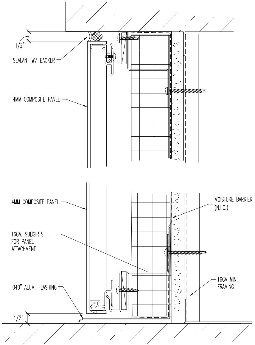
BASE TERMINATION DETAIL
