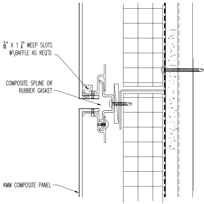
PANEL JOINT DETAIL
